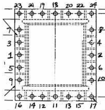
Typical bolt application sequence
